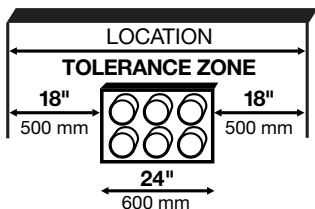
LARGE PIPE OR MULTIPLE DUCTS
